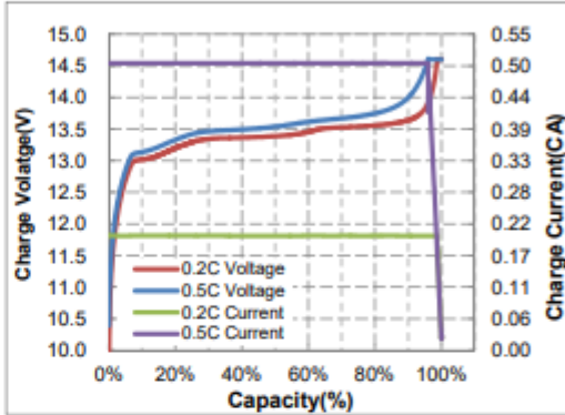
Charge Characteristics of time-voltage@0.2C&0.5C, 25°C
