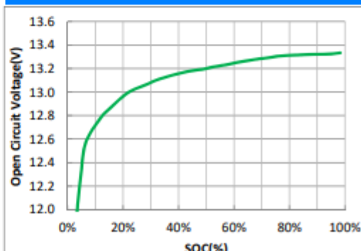
Open circuit voltage VS SOC%@25°C
